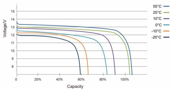
Charge & Discharge Voltage Characteristics
